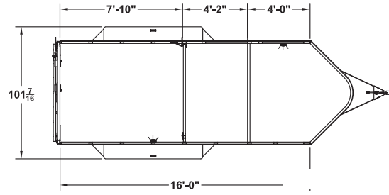
EXPRESS STC 616 BP FLOORPLAN (6'8" Tall Shown) 7'2" Tall
