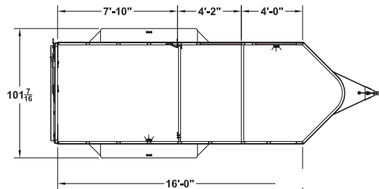
EXPRESS STC 616 BP FLOORPLAN 7'2" Tall
